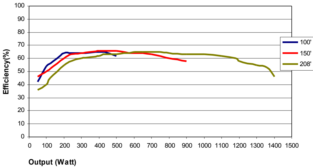
Efficiency of LV1500
