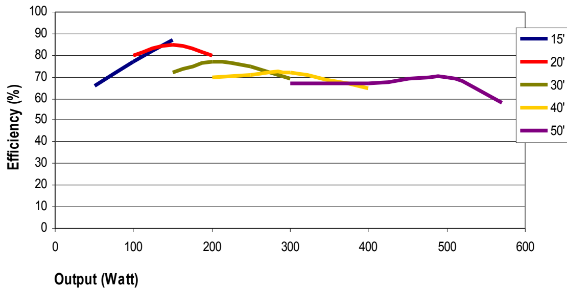
Efficiency of LV750 w. 2 Nozzles
